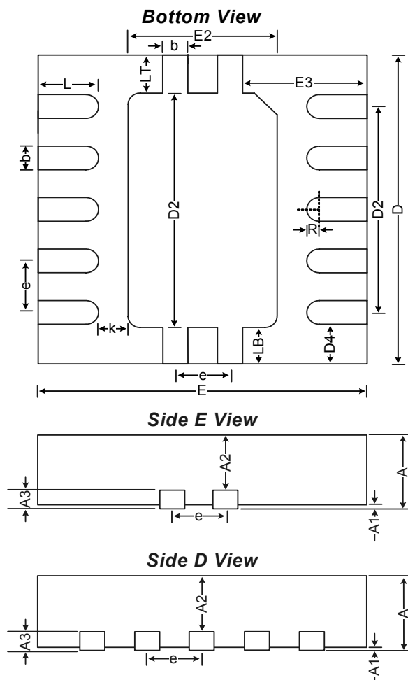
Figure 5. QFN-11 Package Drawing
