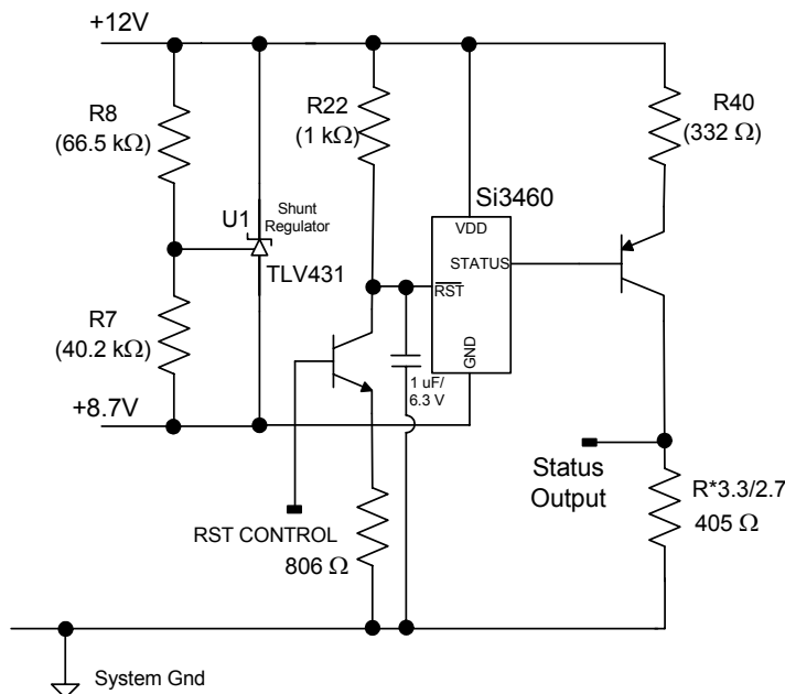
Figure 4. STATUS and RESET Pin Interface when Referenced to System Ground
