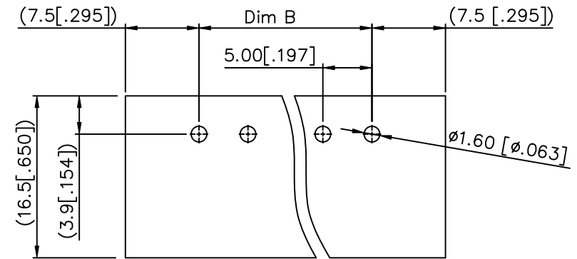
PCB LAYOUT
