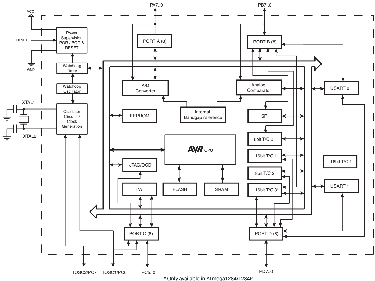
Figure 2-1. Block diagram.
