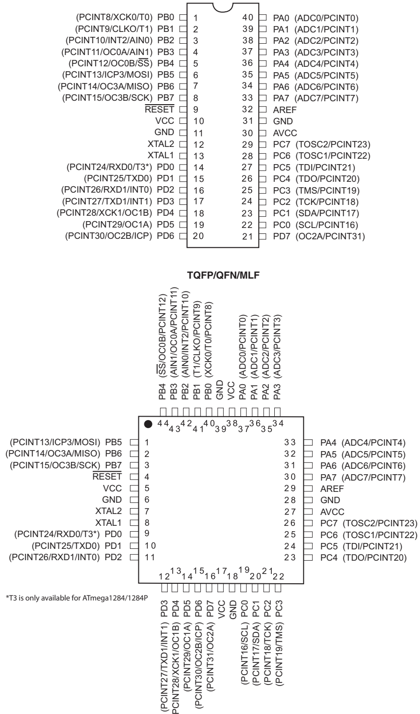
Figure 1-1. Pinout.
