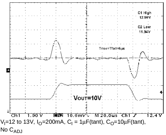
Figure 26: Line Transient
