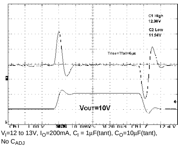
Figure 24: Line Transient
