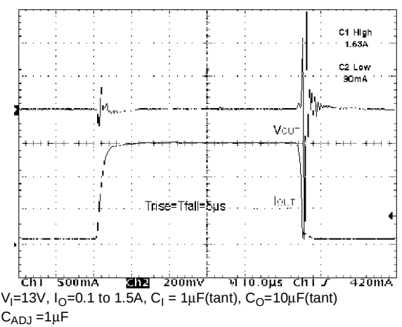
Figure 27: Load Transient
