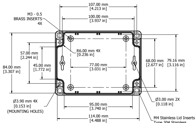
BOX - INSIDE
