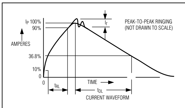
Figure 8b. Human Body Model Current Waveform
