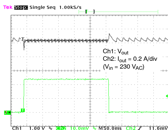
Figure 35. Charger Load Transient Response
