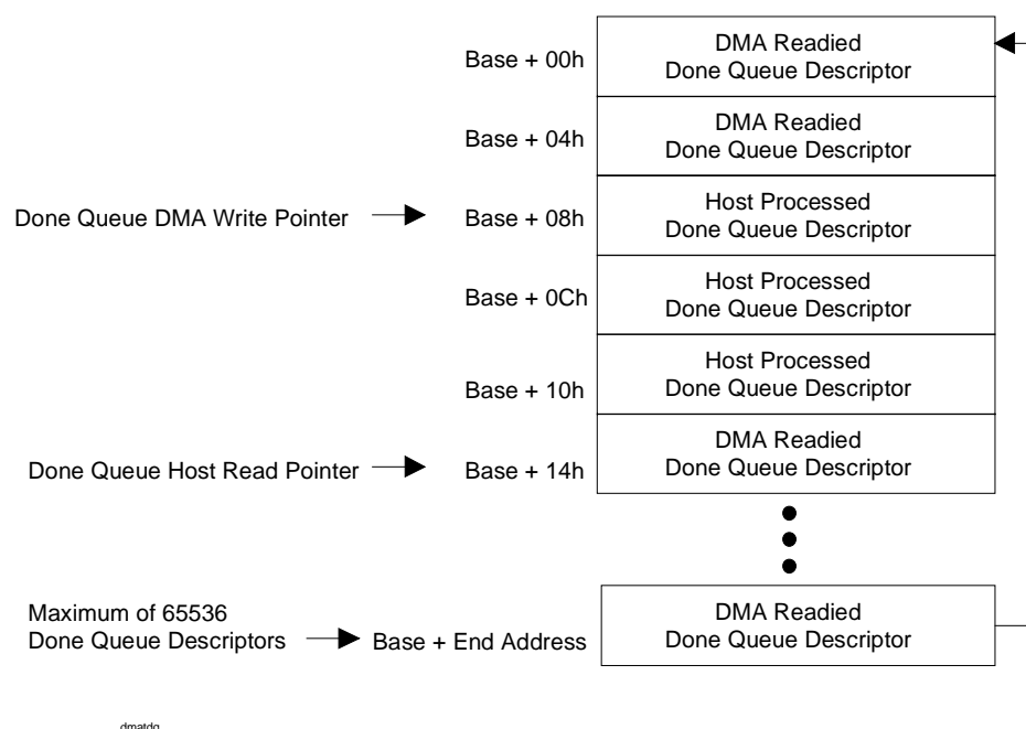
Transmit Done Queue Structure Figure 8.2.4B
