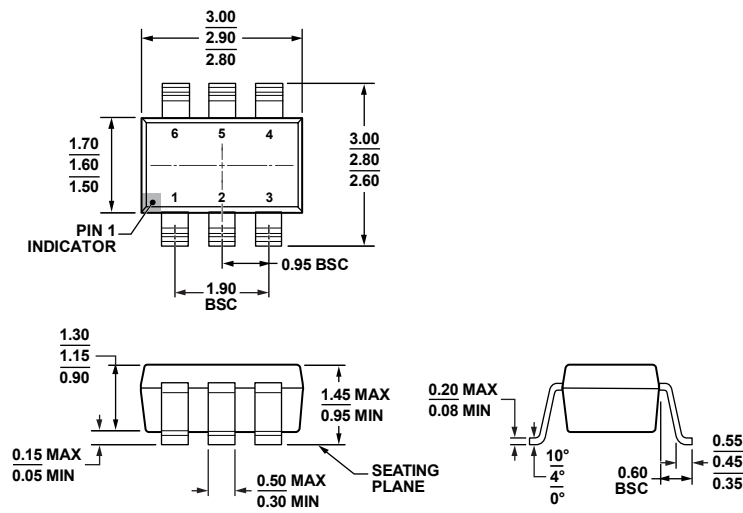
Figure 21. 6-Lead Small Outline Transistor Package [SOT-23] (RJ-6)
