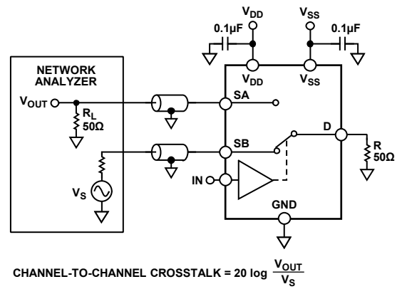
Figure 35. Channel-to-Channel Crosstalk
