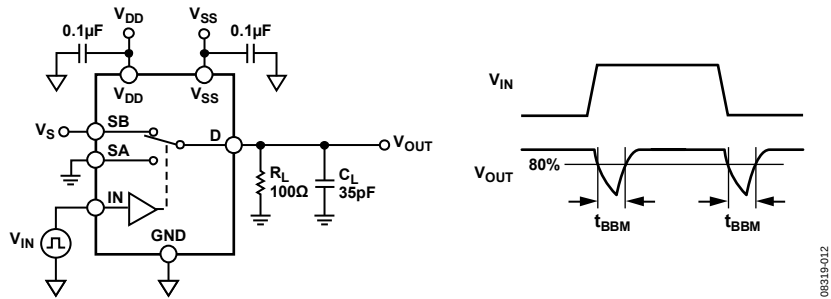
Figure 30. Break-Before-Make Delay, t_D
