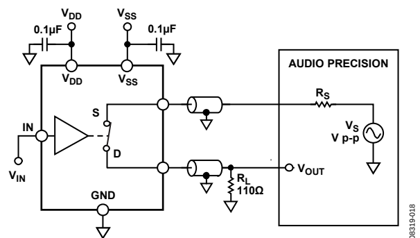
Figure 36. THD + Noise
