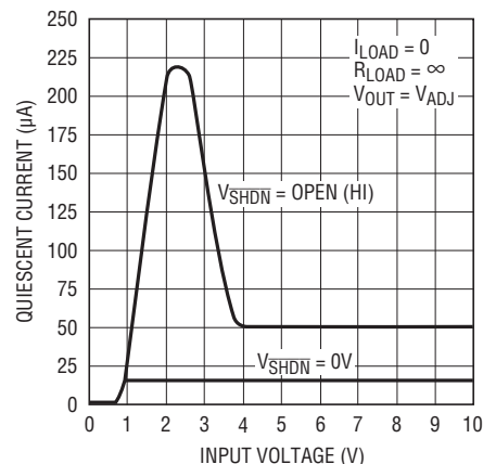
LT1129 Quiescent Current
