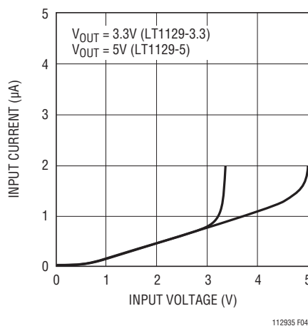
Figure 4. Input Current
