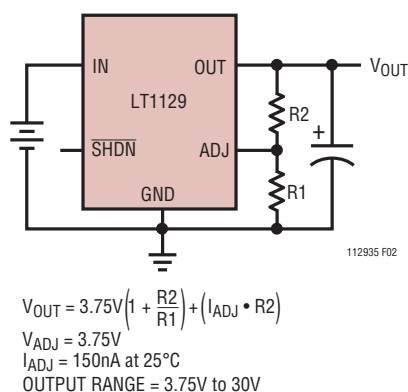
Figure 2. Adjustable Operation
