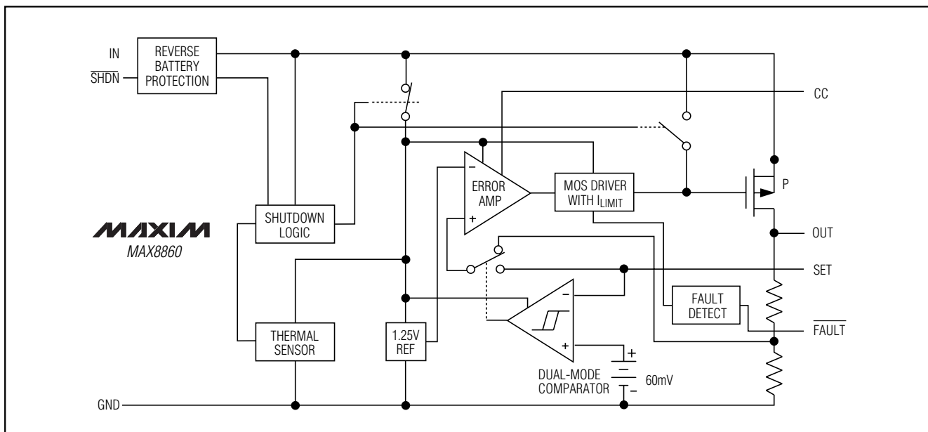
Figure 1. Functional Diagram
