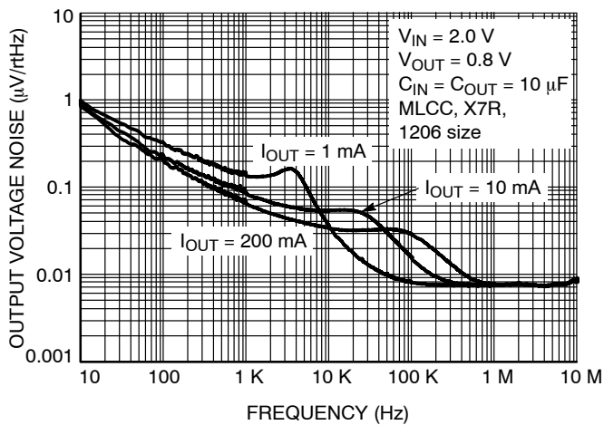
Figure 5. Output Voltage Noise Spectral Density for V_{\text{OUT}} = 0.8 \text{ V} , C_{\text{OUT}} = 10 \mu\text{F}
