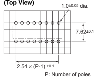
PCB Dimensions (Top View)
