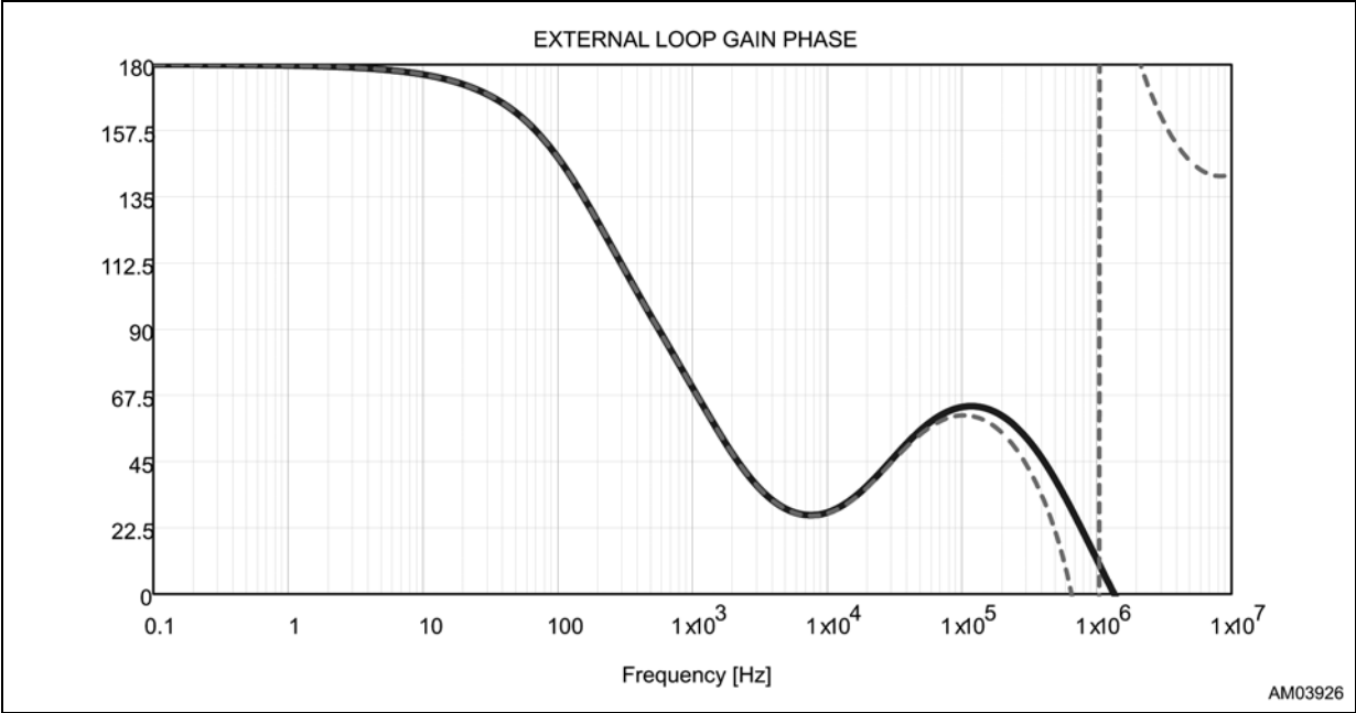
Figure 57. Phase Margin Bode's plot of A6985F (V OUT = 6 V) evaluation board
