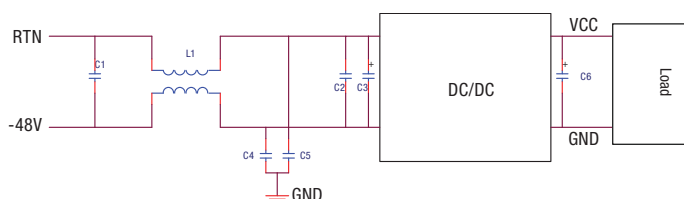
Figure 2. Conducted Emissions Test Circuit
