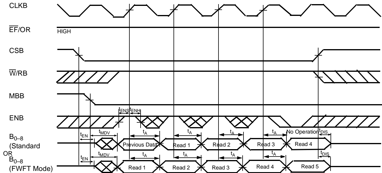
Port B Word Read Cycle Timing for FIFO (CY Standard and FWFT Modes) [17]
