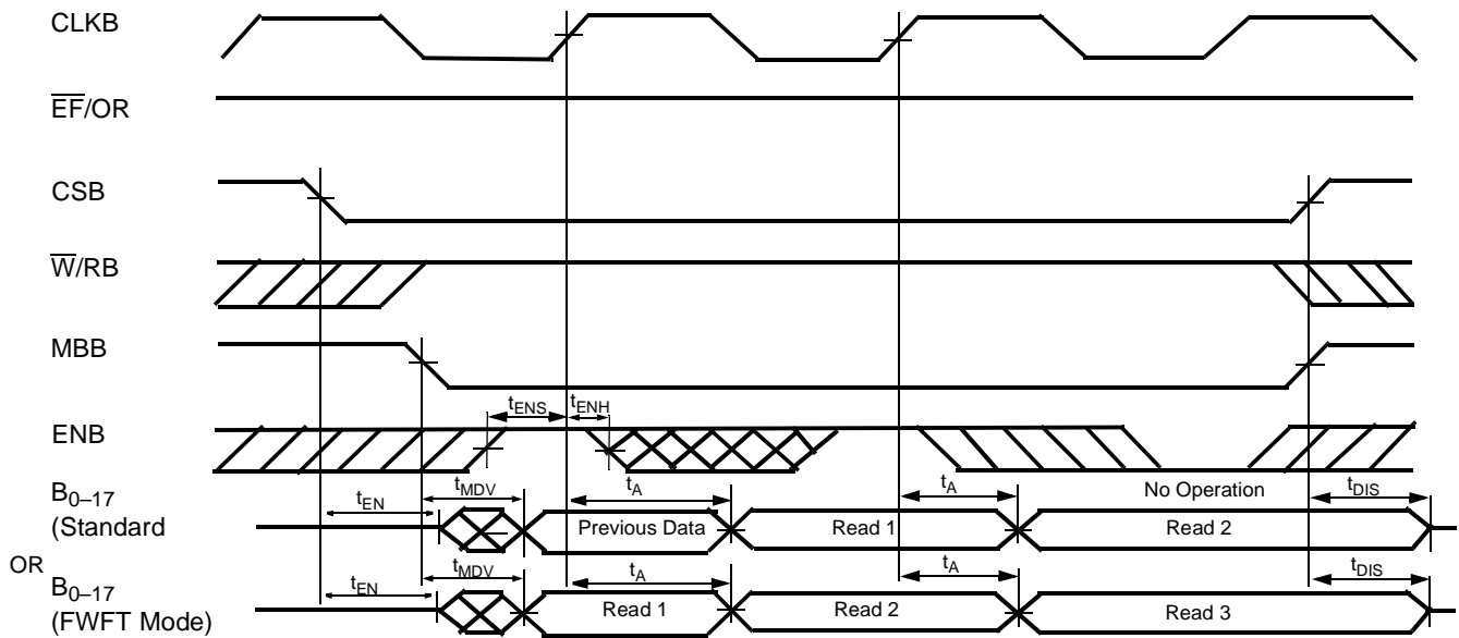
Port B Byte Read Cycle Timing for FIFO (CY Standard and FWFT Modes) [18]
