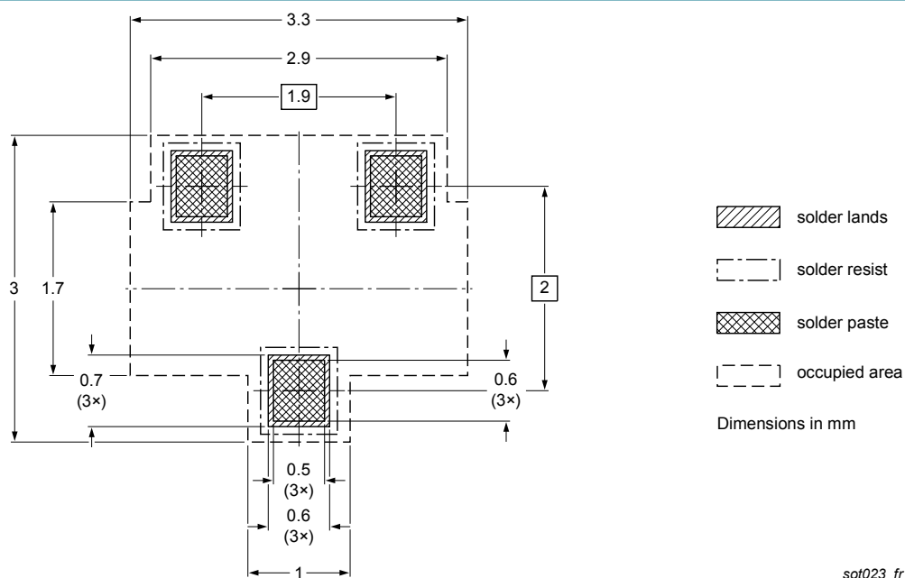
Fig. 12. Reflow soldering footprint for TO-236AB (SOT23)
