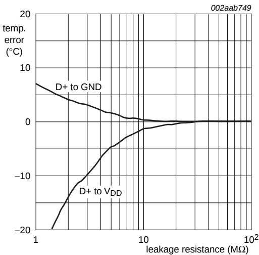
Fig 7. Temperature error versus printed-circuit board leakage resistance
