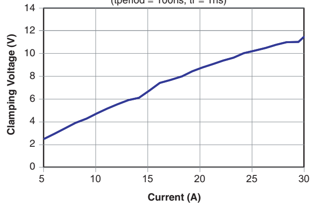
Clamping Voltage vs. Current ( t_{period} = 100ns , t_r = 1ns )
