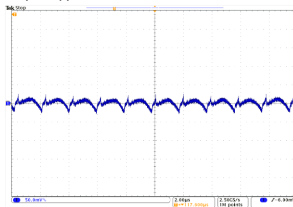
Output Ripple: 24Vin, 3.3Vout at 15A
