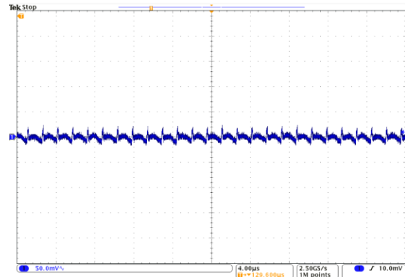
Output Ripple: 24Vin, 2.5Vout at 15A
