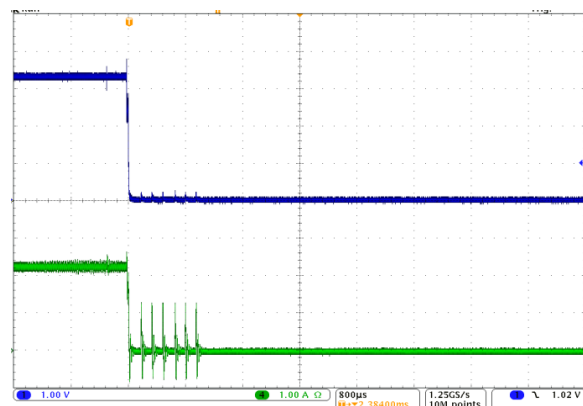
Short Circuit
