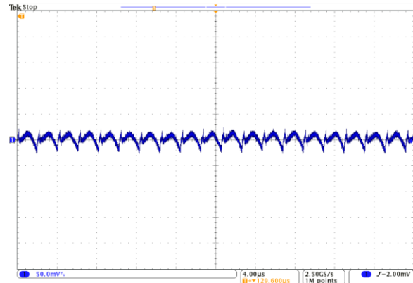
Output Ripple: 24Vin, 2.5Vout at 7.5A
