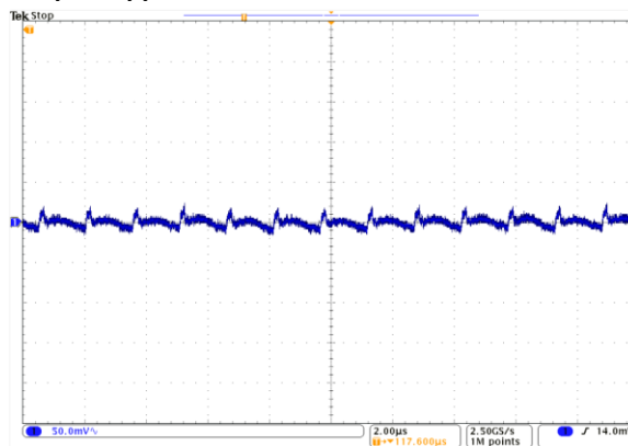
Output Ripple: 24Vin, 3.3Vout at 7.5A
