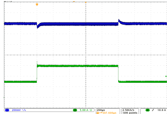
Transient Response: 7.5A to 15A, at 5A/μs
