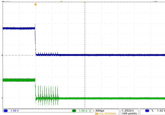
Short Circuit
