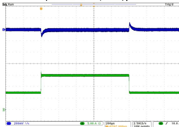
Transient Response: 7.5 to 15A, at 5A/μs
