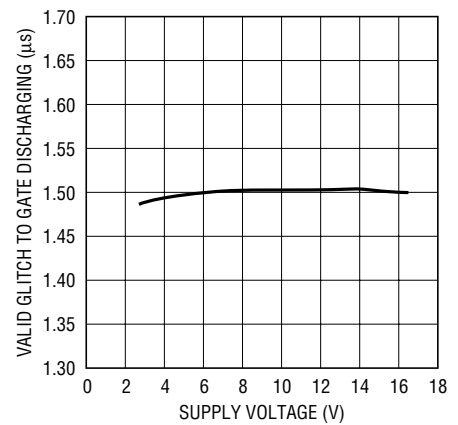
Valid Glitch to GATE Discharging vs Supply Voltage
