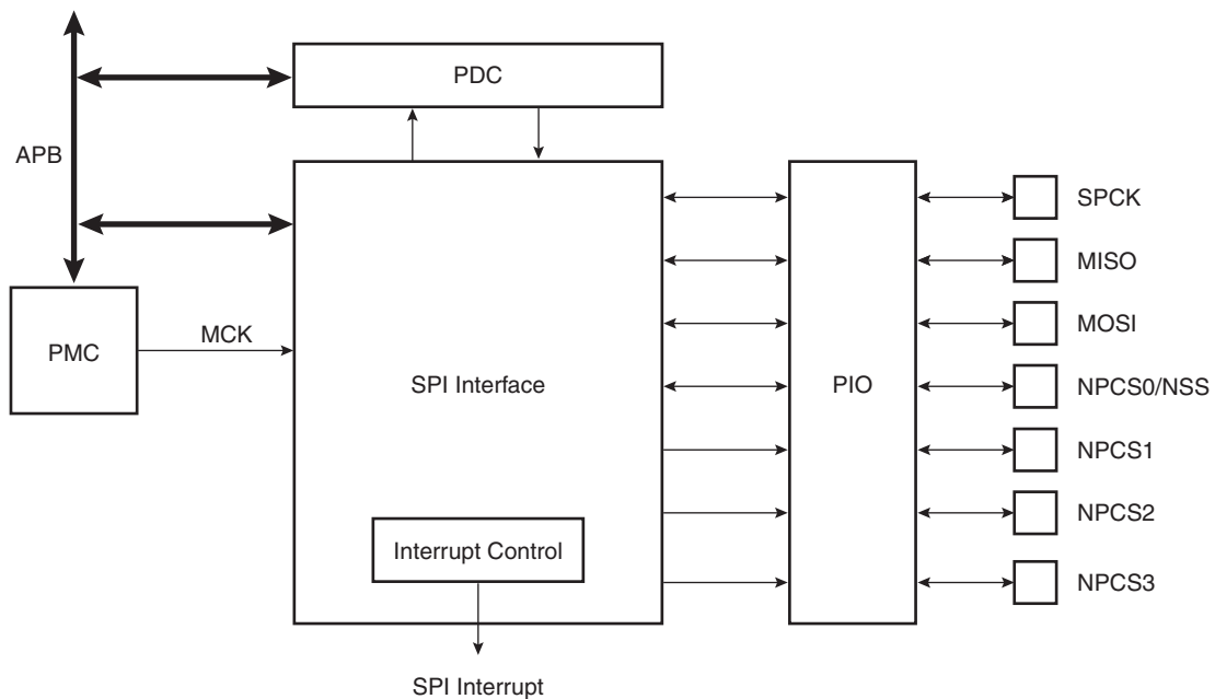
Figure 30-1. Block Diagram
