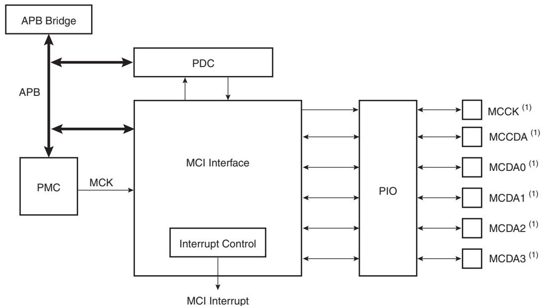
Figure 35-1. Block Diagram
