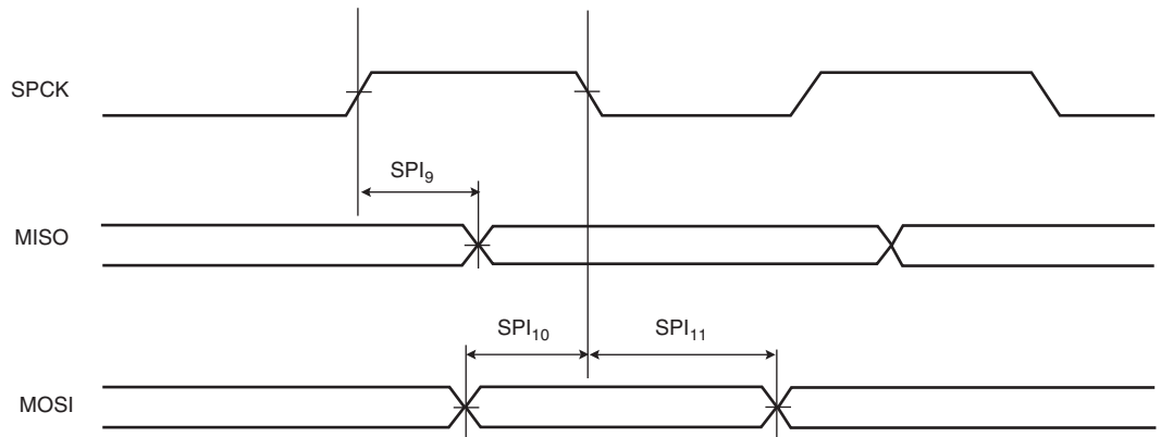
Figure 39-10. SPI Slave mode with (CPOL = NCPHA = 0) or (CPOL= NCPHA= 1)
