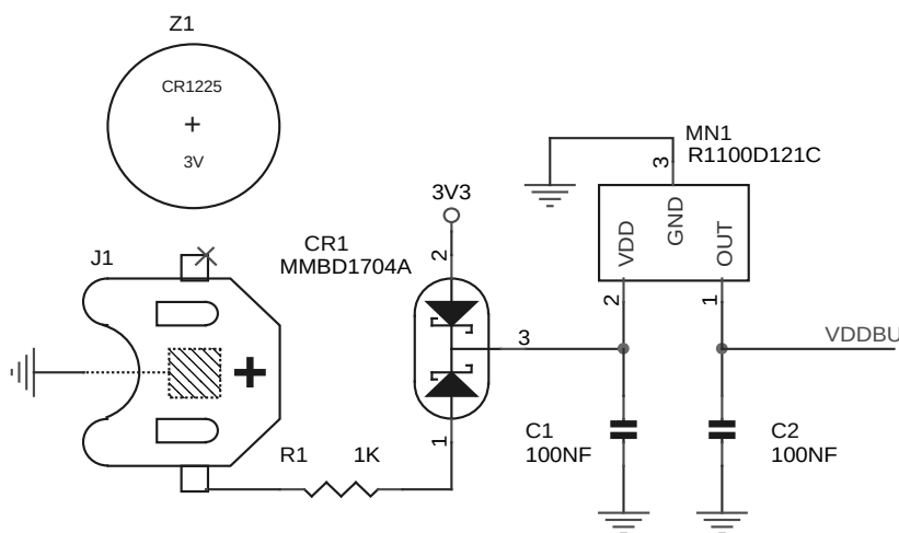
Figure 42-1. Schematic
