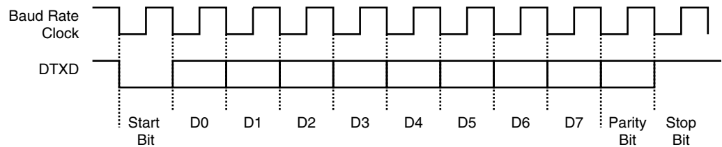
Figure 28-10. Character Transmission
