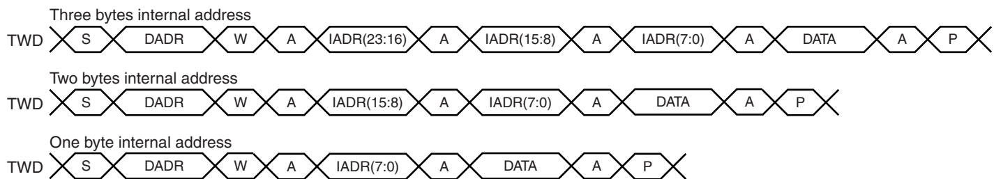
Figure 31-10. Master Write with One, Two or Three Bytes Internal Address and One Data Byte
