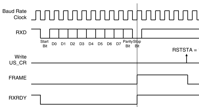
Figure 32-15. Framing Error Status
