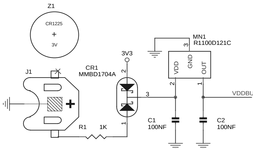
Figure 42-2. Schematic
