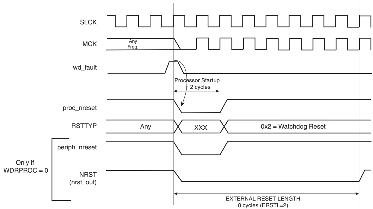
Figure 14-8. Watchdog Reset
