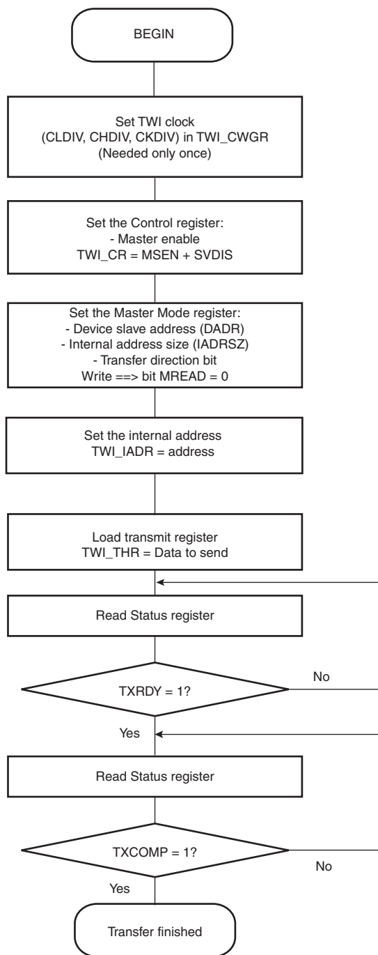
Figure 31-14. TWI Write Operation with Single Data Byte and Internal Address
