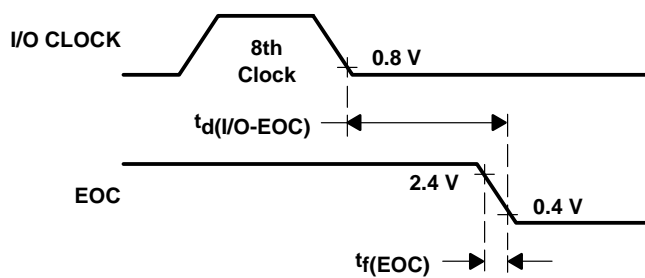
Figure 6. EOC Timing
