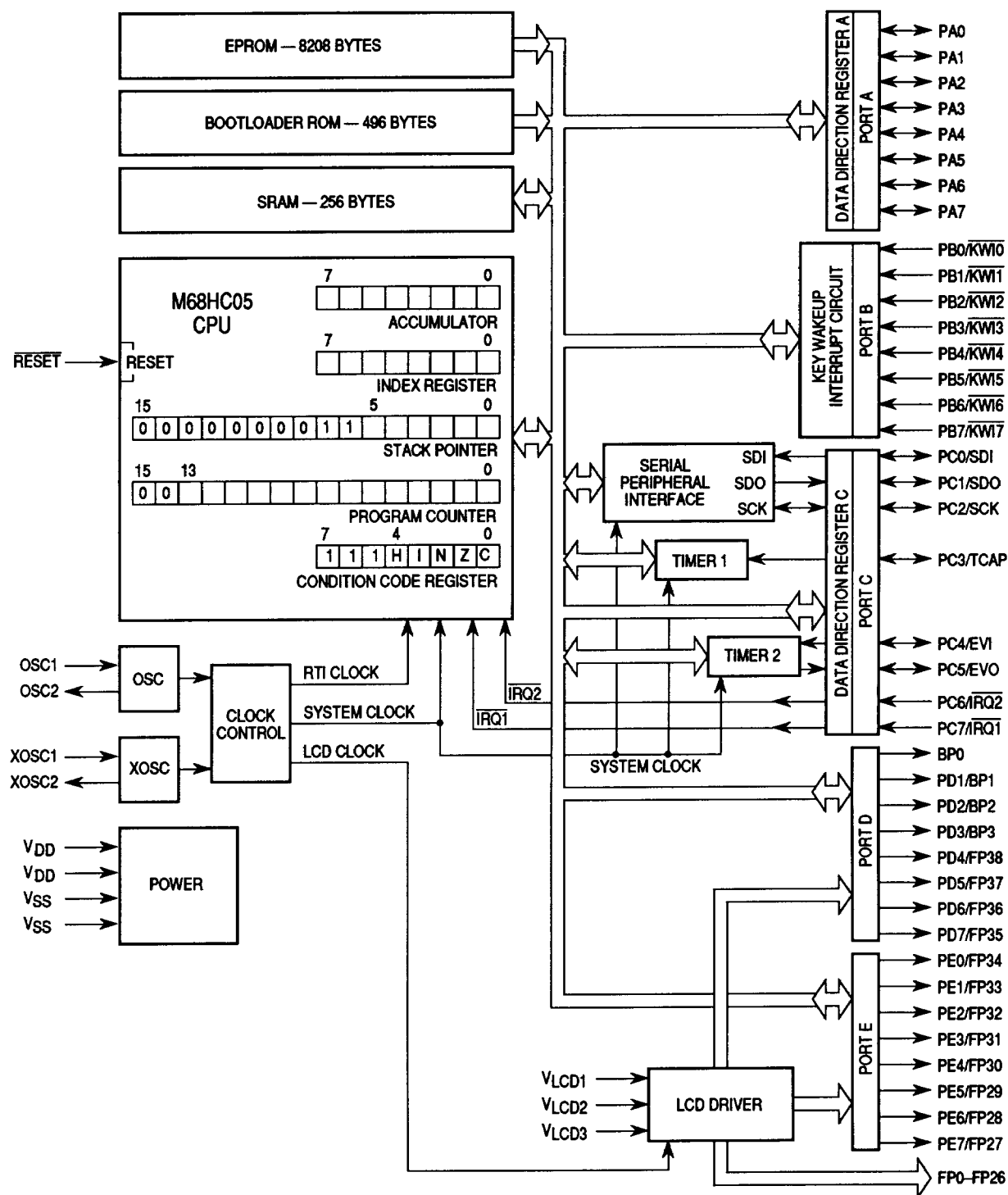
MCU Structure
