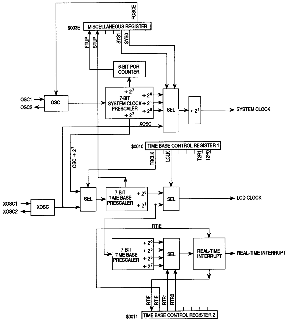
Clock Distribution
