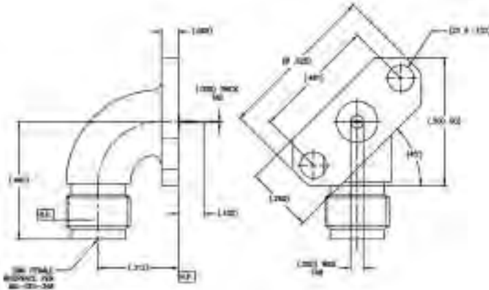
Tensolite Part No. Flange Angle Tab Position 5645 45° Right Horizontal 5646 45° Left Horizontal 5651 45° Right Vertical 5652 45° Left Vertical
