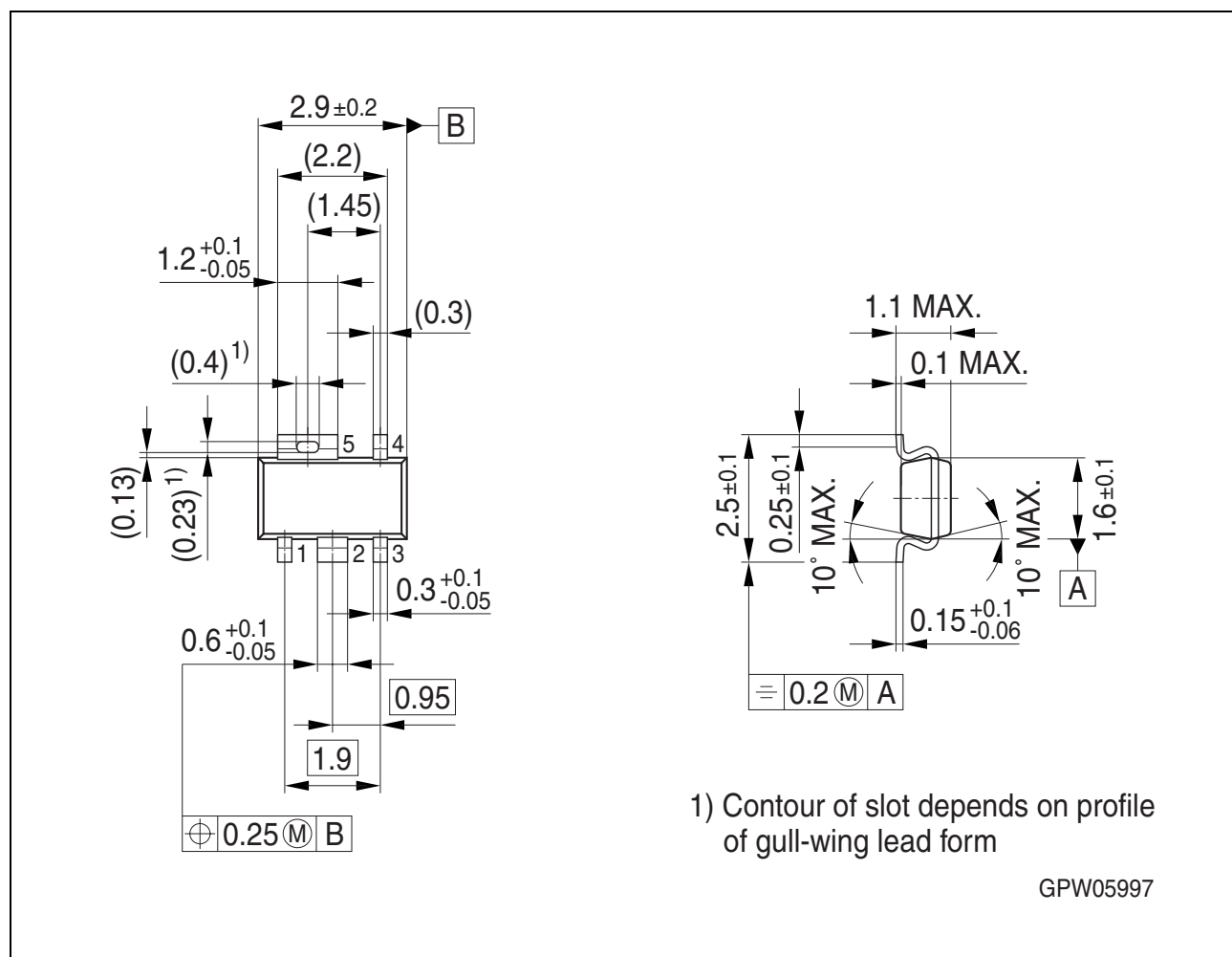
Figure 4 Outline PG-SCT595-5
