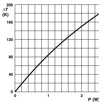
Ø 0.78 mm FeCu-leads
