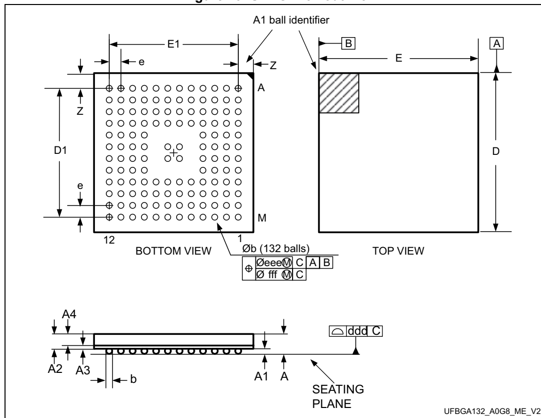
Figure 49. UFBGA132 outline
