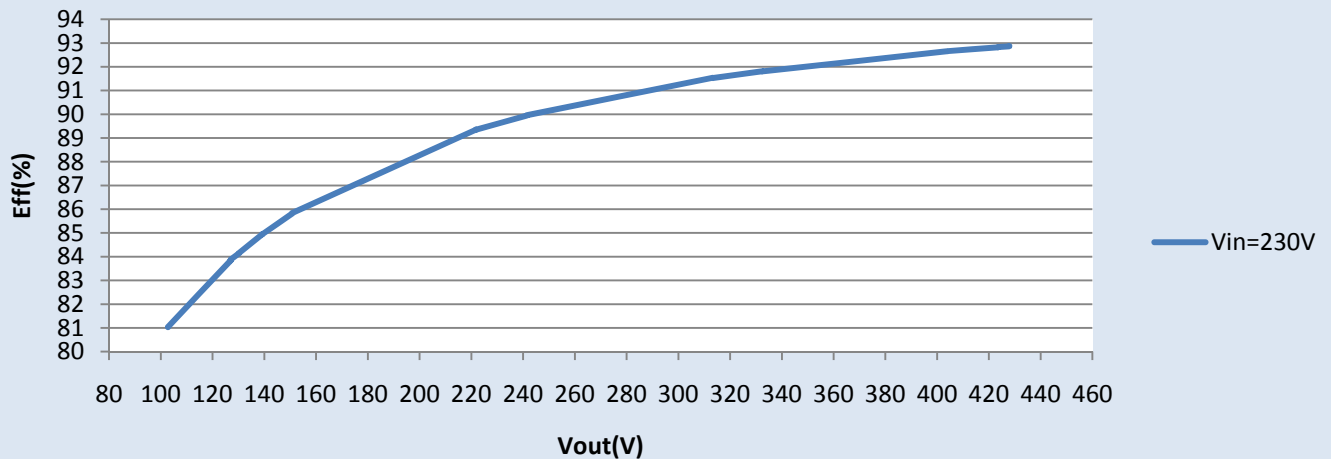
Eff Vs Vout at 80C case
