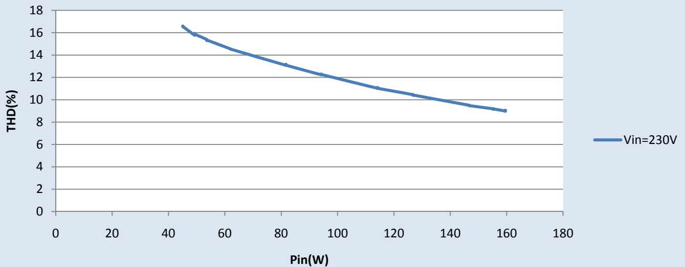
THD Vs Pin at 80C case
