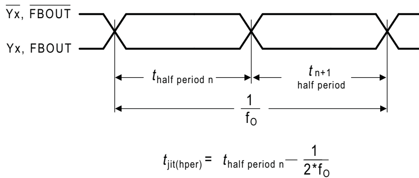
Figure 7. Half-Period Jitter
