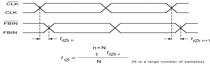
Figure 3. Cycle-to-Cycle Jitter
