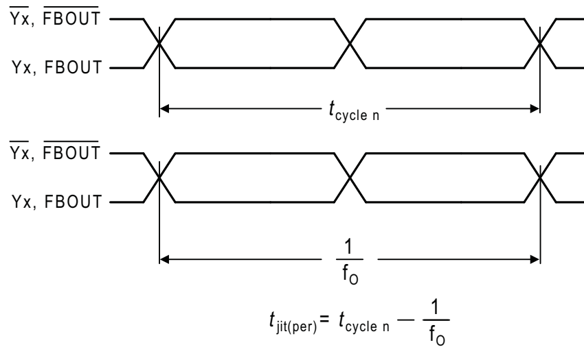
Figure 6. Period Jitter
