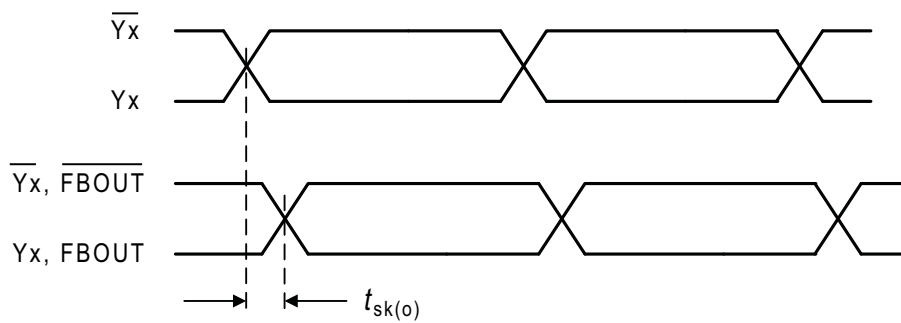
Figure 5. Output Skew
