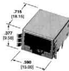
Part Number 1116201-1
