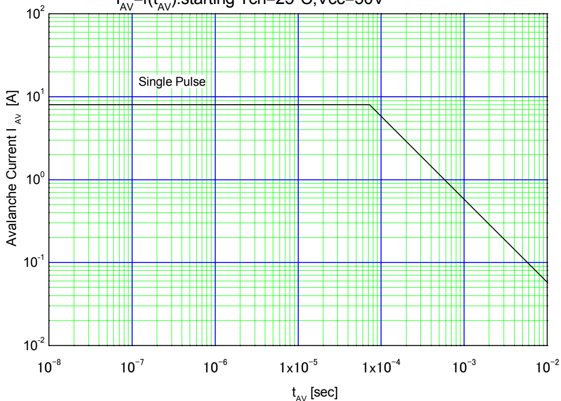
Maximum Avalanche Current Pulsewidth
