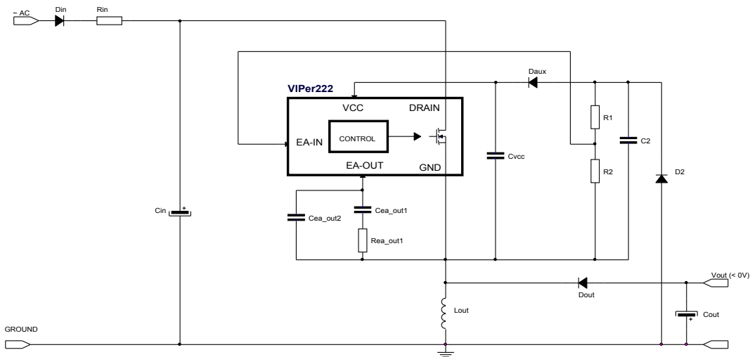
Figure 14. Buck-Boost converter
