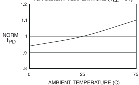
NORMALIZED t_{PD} vs. AMBIENT TEMPERATURE ( V_{CC} = 5V )
