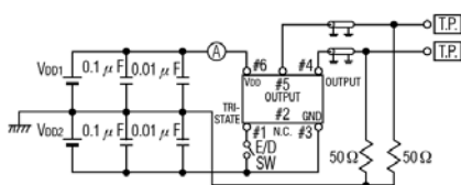
Figure 1) Test Circuit (1)
