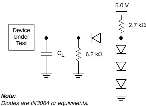
Figure 9. Test Setup
