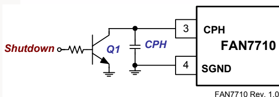
Figure 24. External Shutdown Circuit
