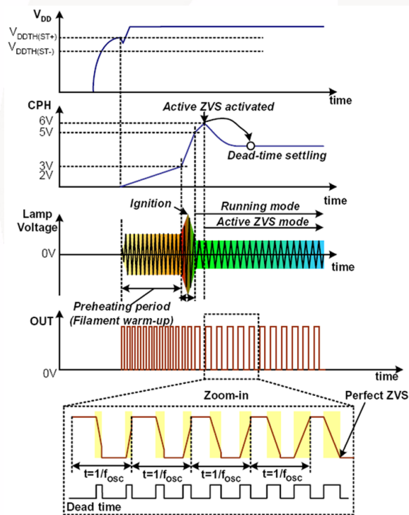
Figure 23. Typical Transient Waveform from Preheating to Active ZVS Mode
