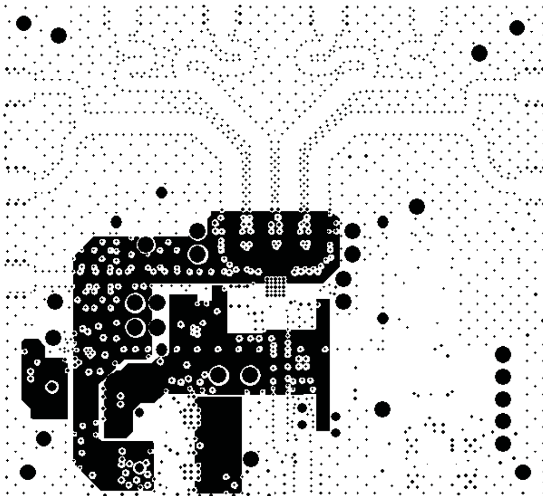
Figure 8. Layer 3, Power
