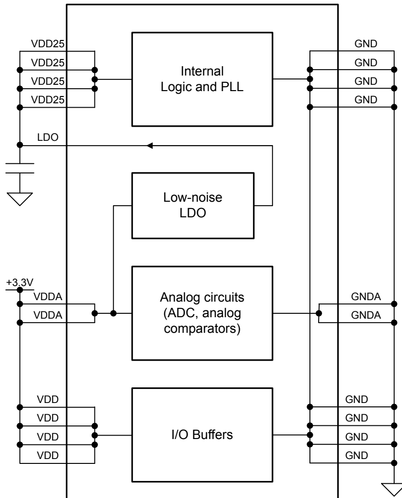
Figure 6-4. Power Architecture
