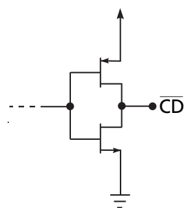
Figure 5-5: \overline{CD} Circuit
