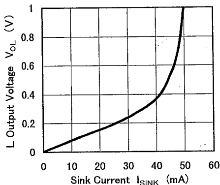
L Output Voltage(OUT Pin) vs. Sink Current ( V^+=6V , OSC: Triangle Waveform V_{P-P}=0.5V , Offset=0.5V, f_{osc}=100kHz , T_a=25^\circ C )
