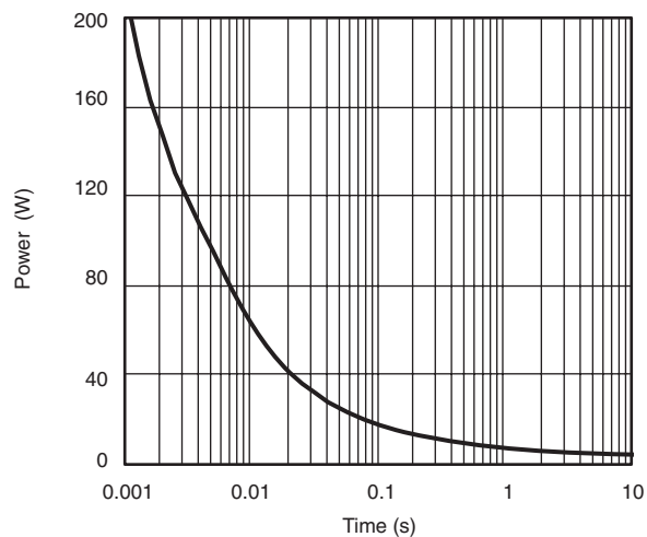
Junction-to-Ambient
