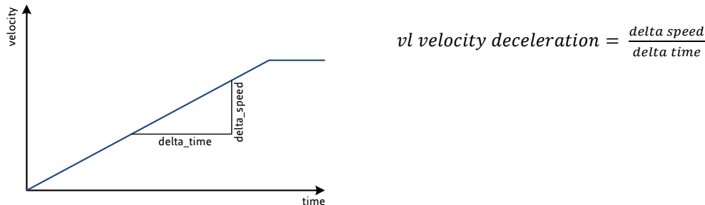
Figure 4.13 Transfer characteristic of the velocity acceleration
