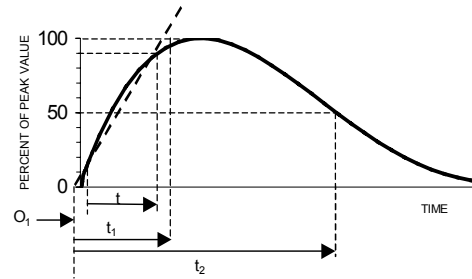
Figure 1: FIGURE 2: PEAK PULSE CURRENT TEST WAVEFORM FOR CLAMPING VOLTAGE
