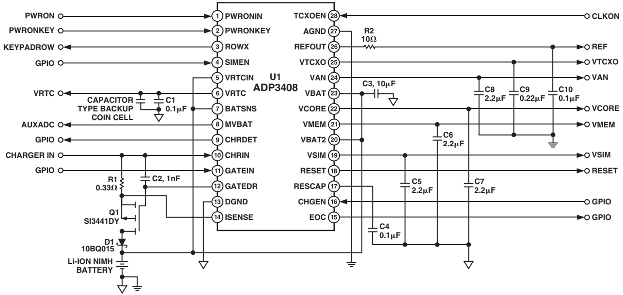
Figure 3a. Typical Application Circuit (TSSOP Option)
