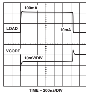
TPC 12. VCORE Load Step
