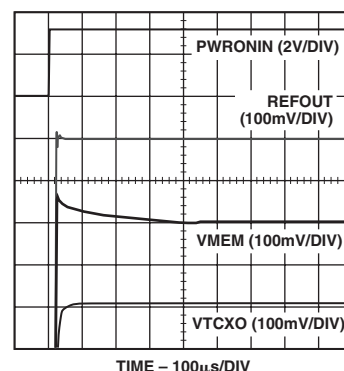
TPC 15. Turn On Transient by PWRONIN, Minimum Load (Part 2)
