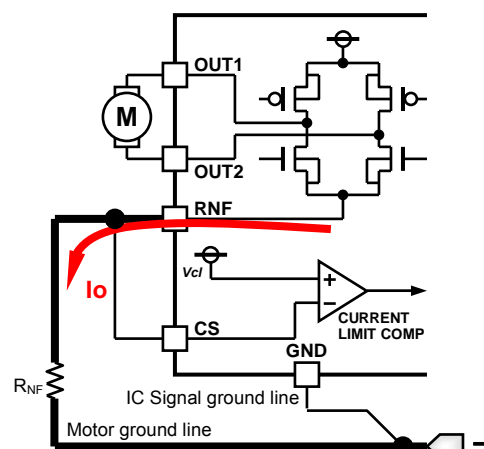
Figure 46. Setting of Current Limit and Ground Lines
