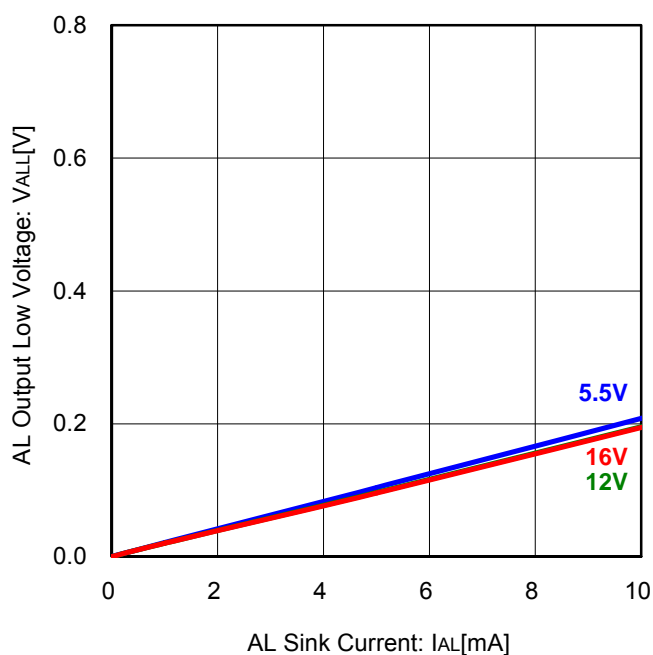
Figure 13. AL Output Voltage vs AL Sink Current ( T_a=25^\circ\text{C} )
