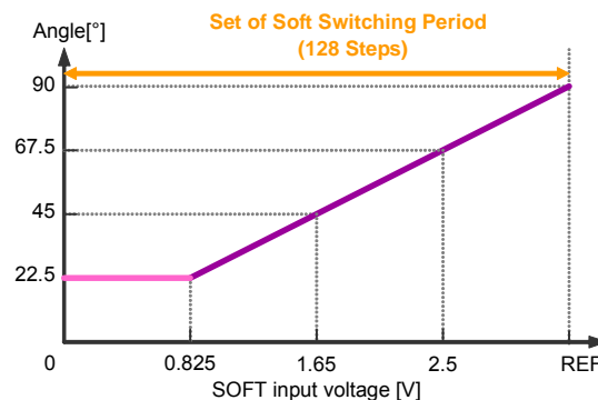
Figure 37. Relation of SOFT Input Voltage and Soft Switching Period
