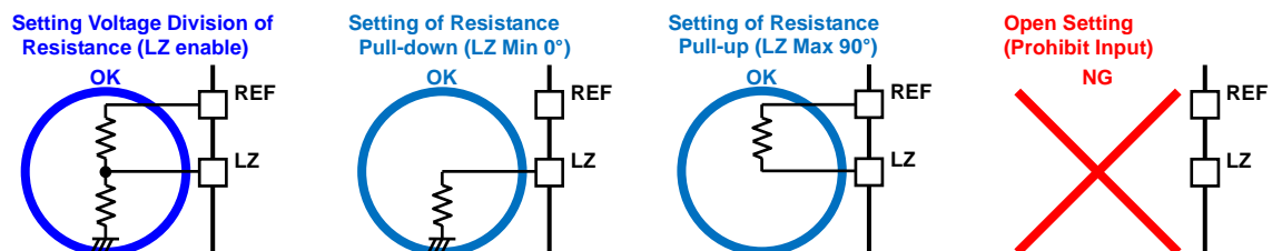
Figure 41. LZ Terminal Setting
