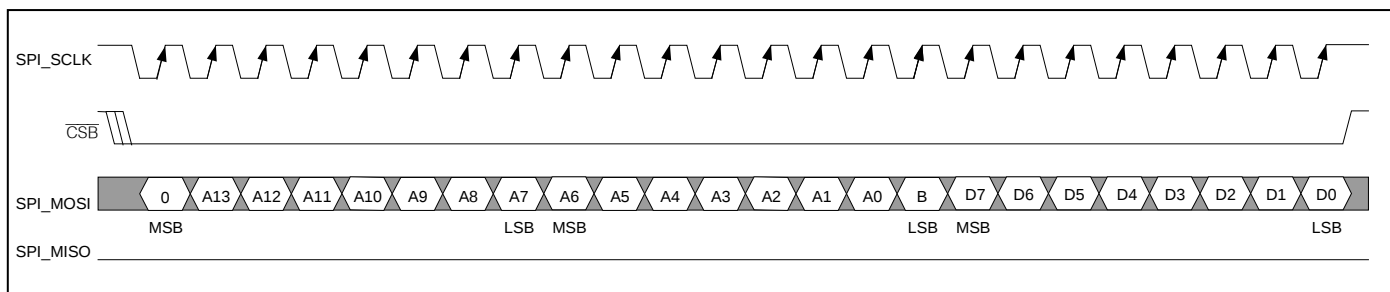
Figure 9-8. SPI Serial Port Access for Write Mode, \text{SPI\_CPOL} = 1 , \text{SPI\_CPHA} = 1
