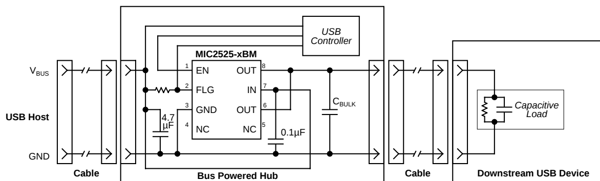
Figure 2. Soft-Start Application
