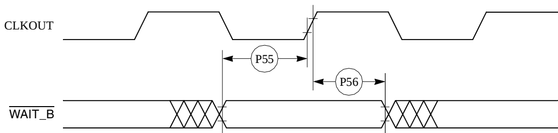
Figure 26. PCMCIA \overline{WAIT\_B} Signal Detection Timing
